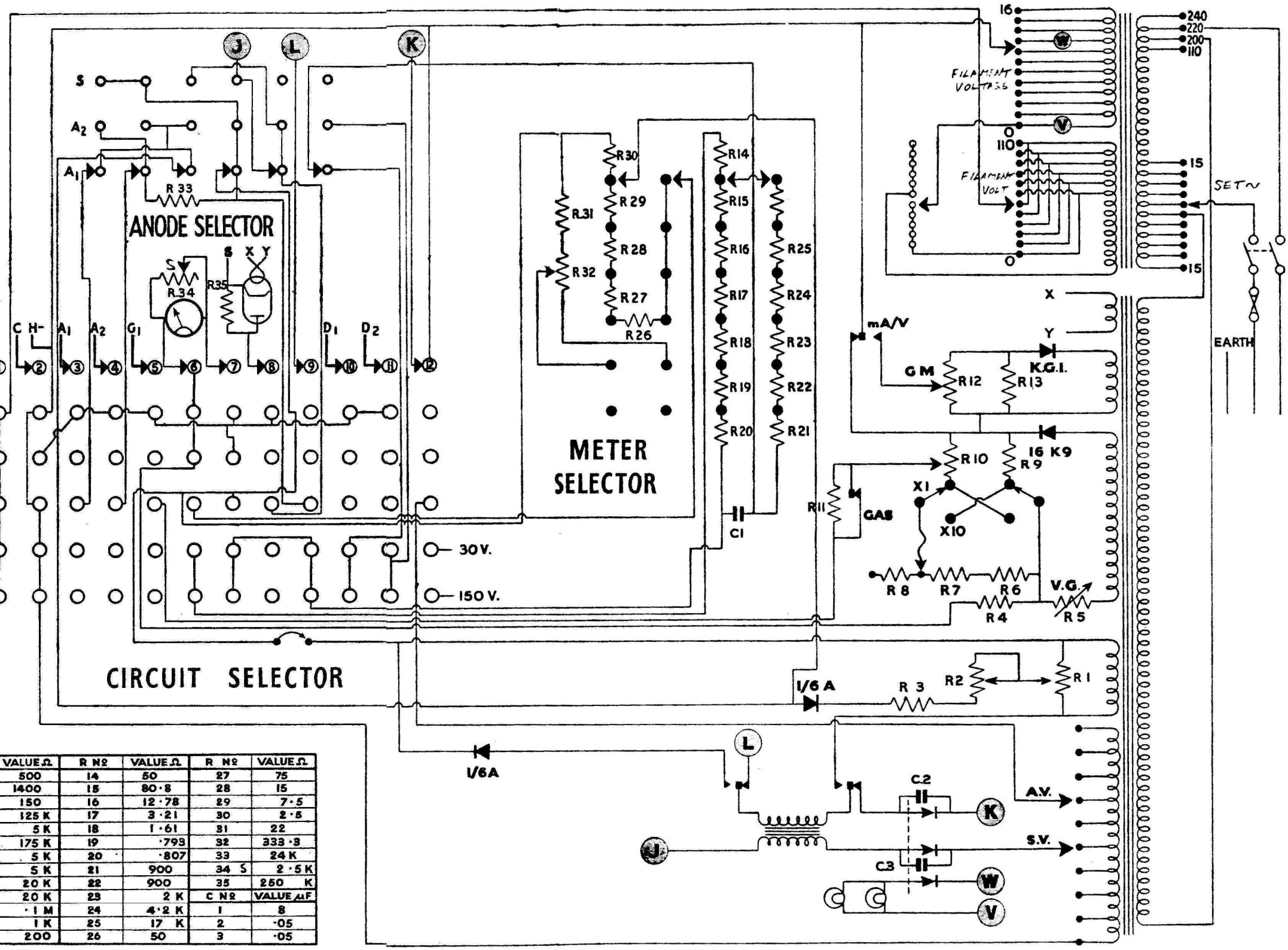
AVO Mk II Valve Tester
